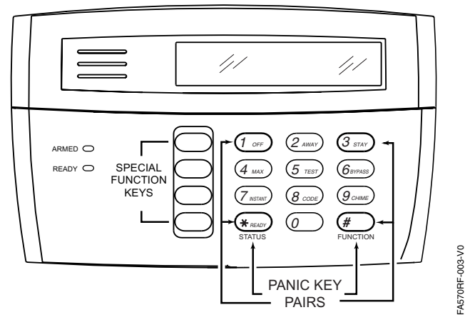
Figure 1. FA570RF Keypad/Transceiver (front door removed)
